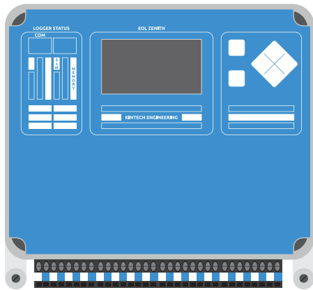
A EOL Zenith data logger with terminal blocks
